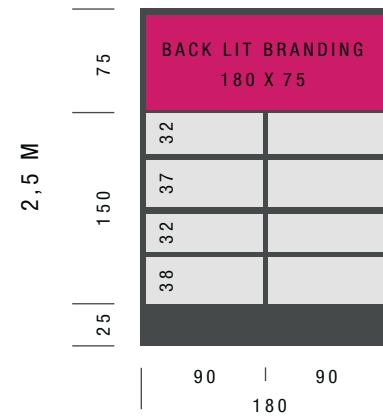
ELEVATION (WITHOUT BAR)
