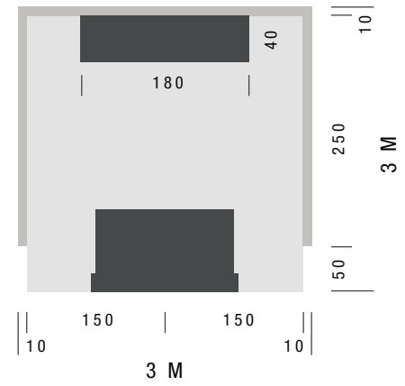
FLOOR PLAN
